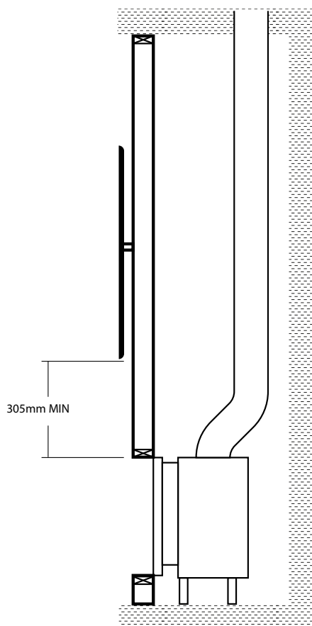
FLUSH INSTALLATION
