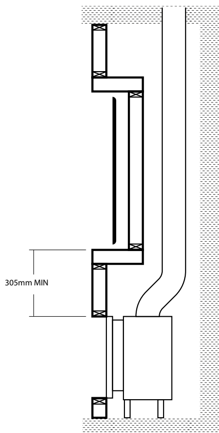
RECESSED INSTALLATION
