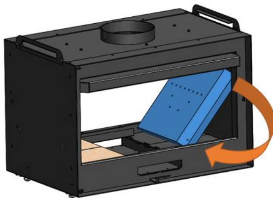
Figure No.17 - Turn the right-side refractory as in the picture so that the deflector can fall
