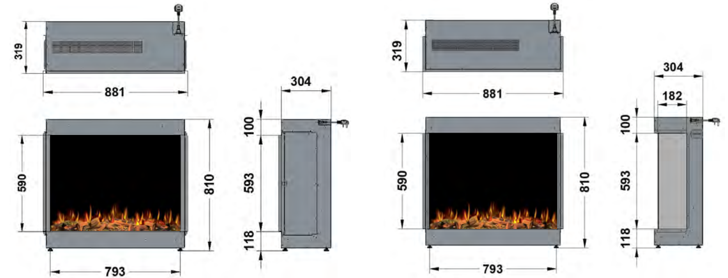
950 ASPECT - BAY
