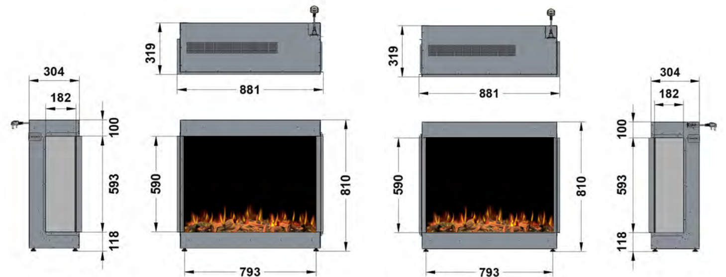
950 ASPECT - FRONT
